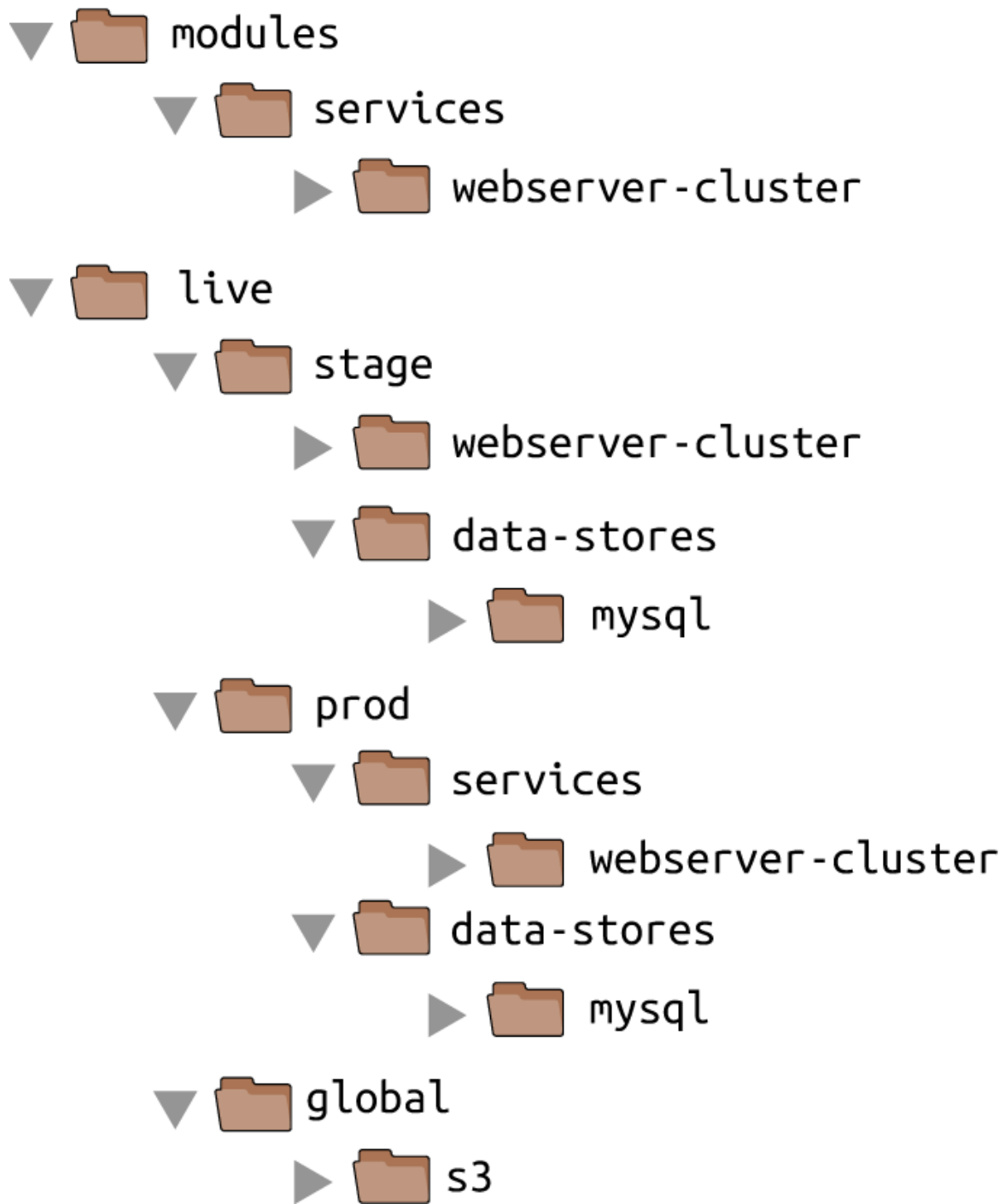
Figure 4-6. File layout with multiple repositories
